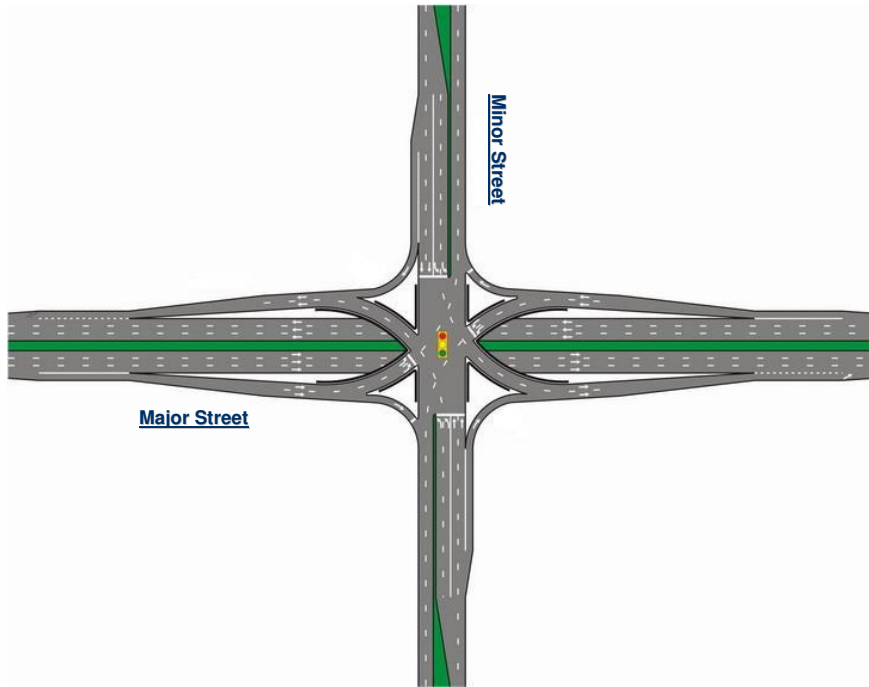
Single Point Interchange (SPUI) (Grade Separated)
